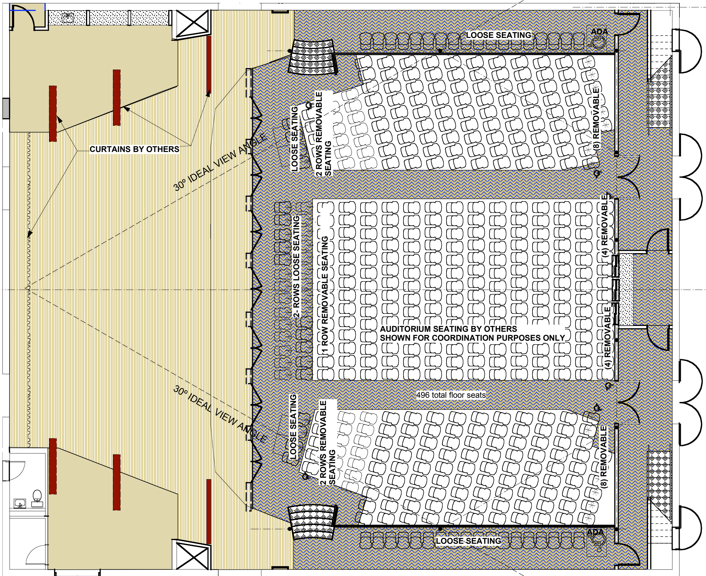
3 SEATING LAYOUT PLAN A1.1 Scale: 1/8" = 1'-0"
